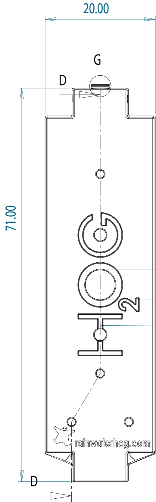
FRONT VIEW
